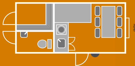
the Mobi – floorplan (16' x 7'6")
